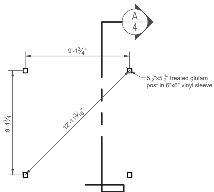
Post Layout Plan
