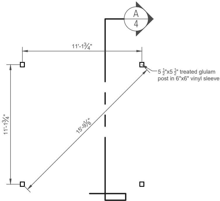
Post Layout Plan
