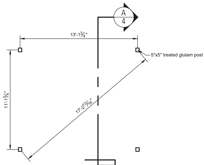
Post Layout Plan
