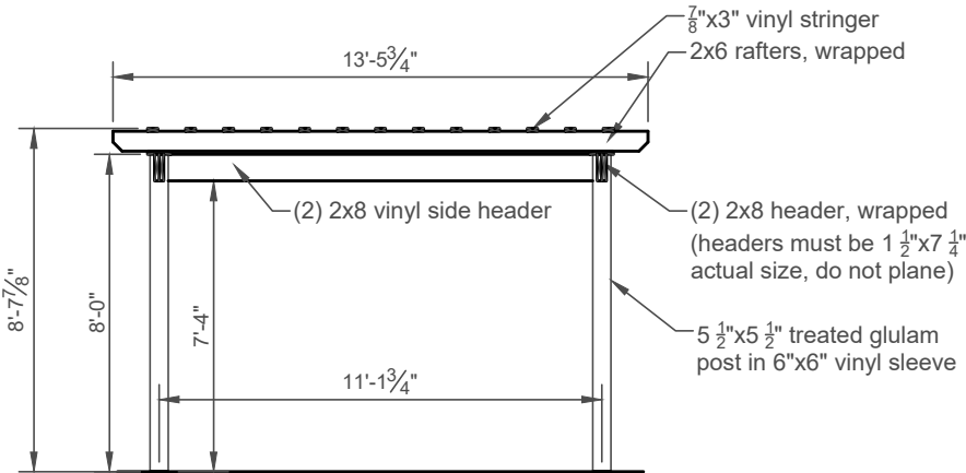
Cross Section A/4 NTS
