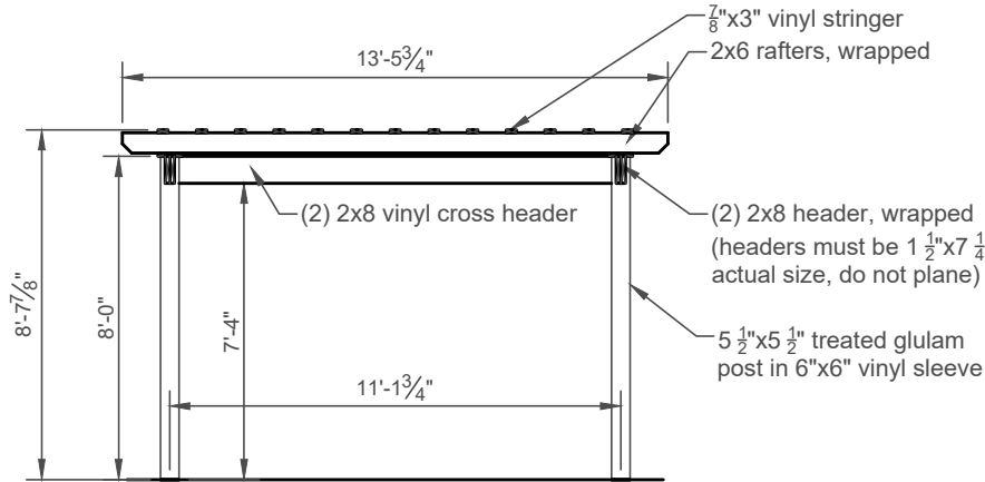
Cross Section B/4 NTS
