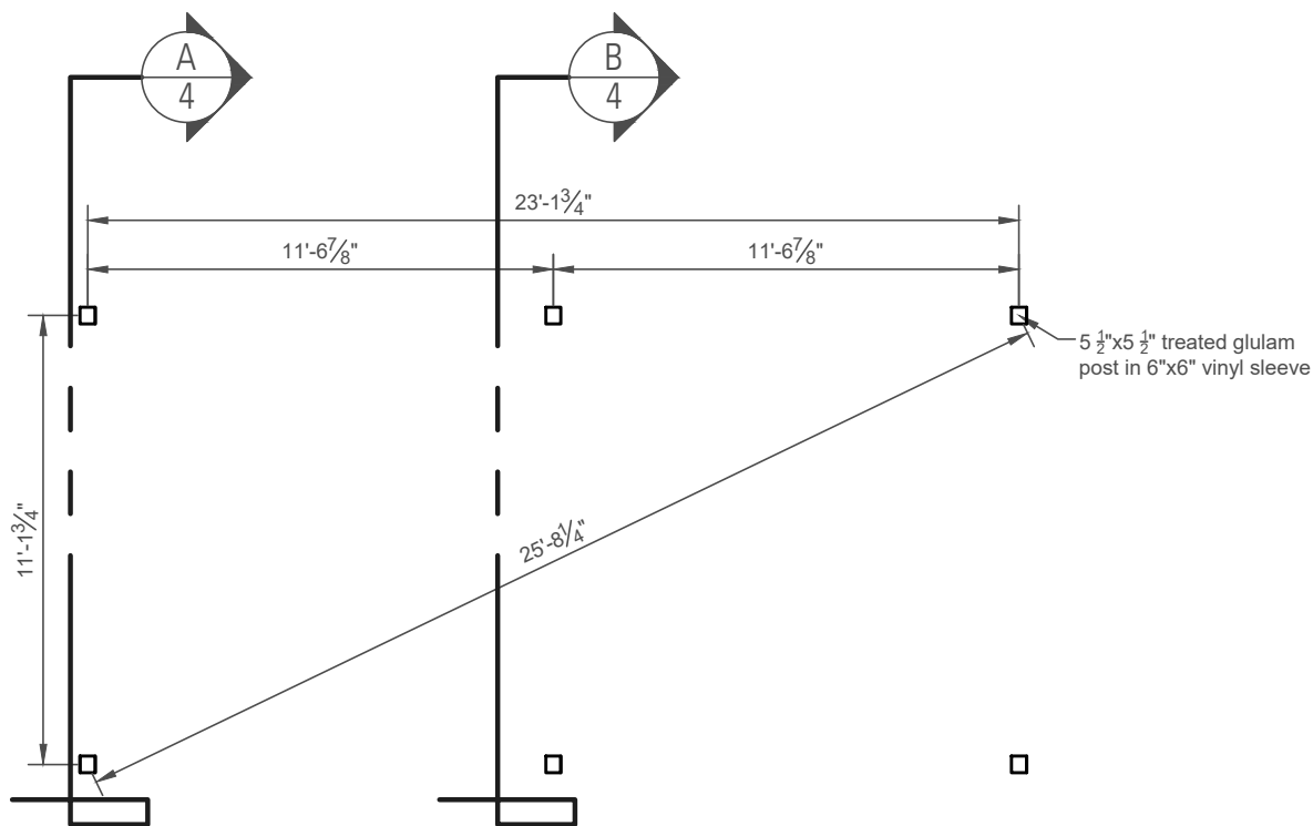
Post Layout Plan NTS
