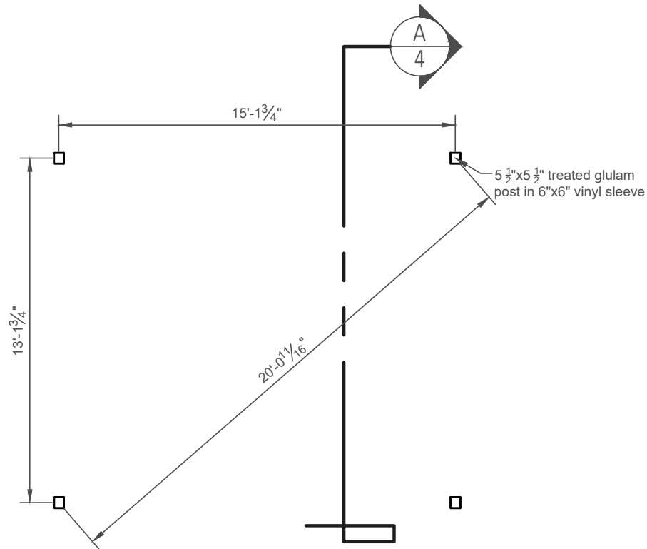
Post Layout Plan
