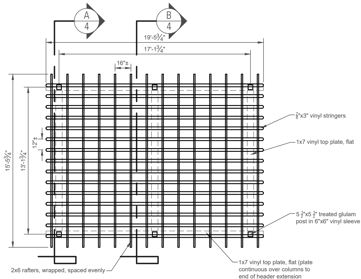
Roof Framing Plan NTS
