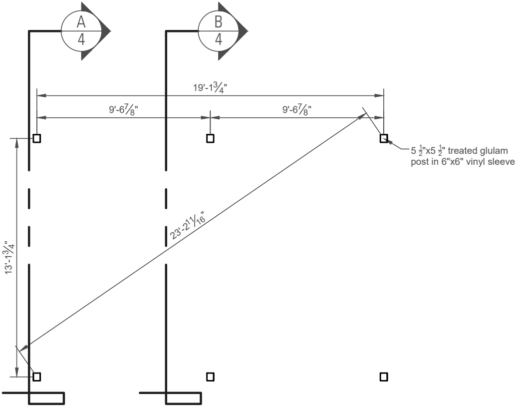
Post Layout Plan
