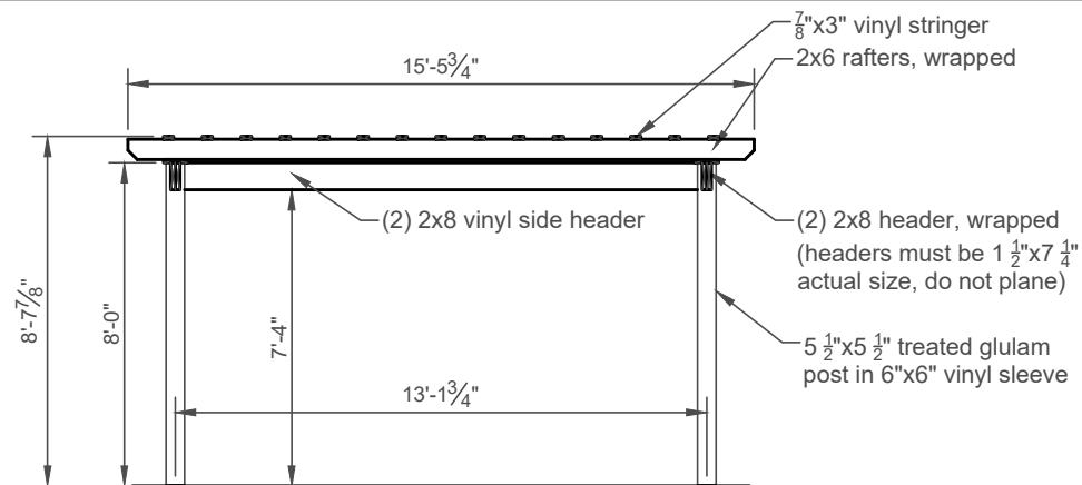
Cross Section A/4 NTS
