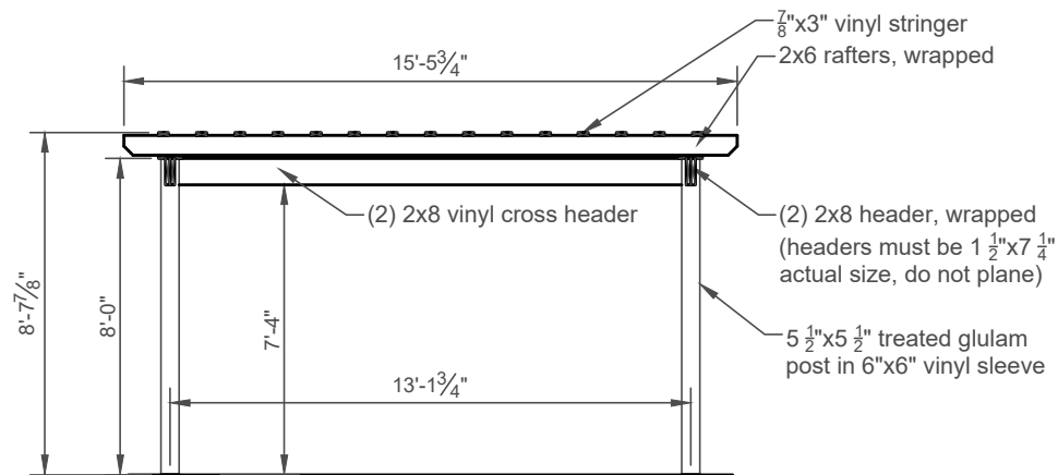
Cross Section B/4 NTS
