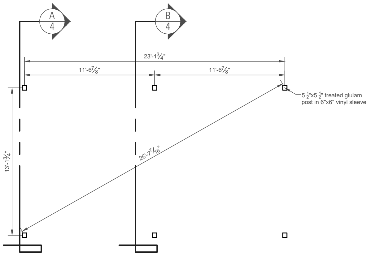
Post Layout Plan
