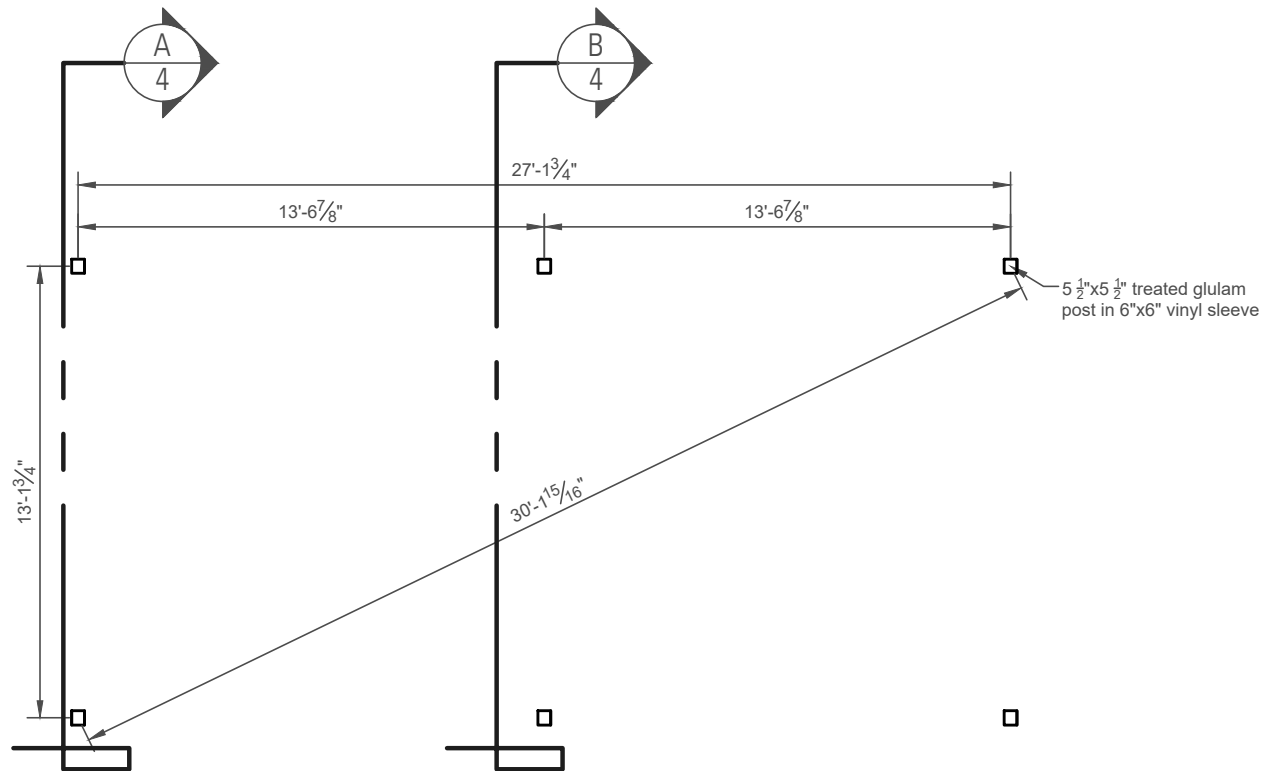
Post Layout Plan
