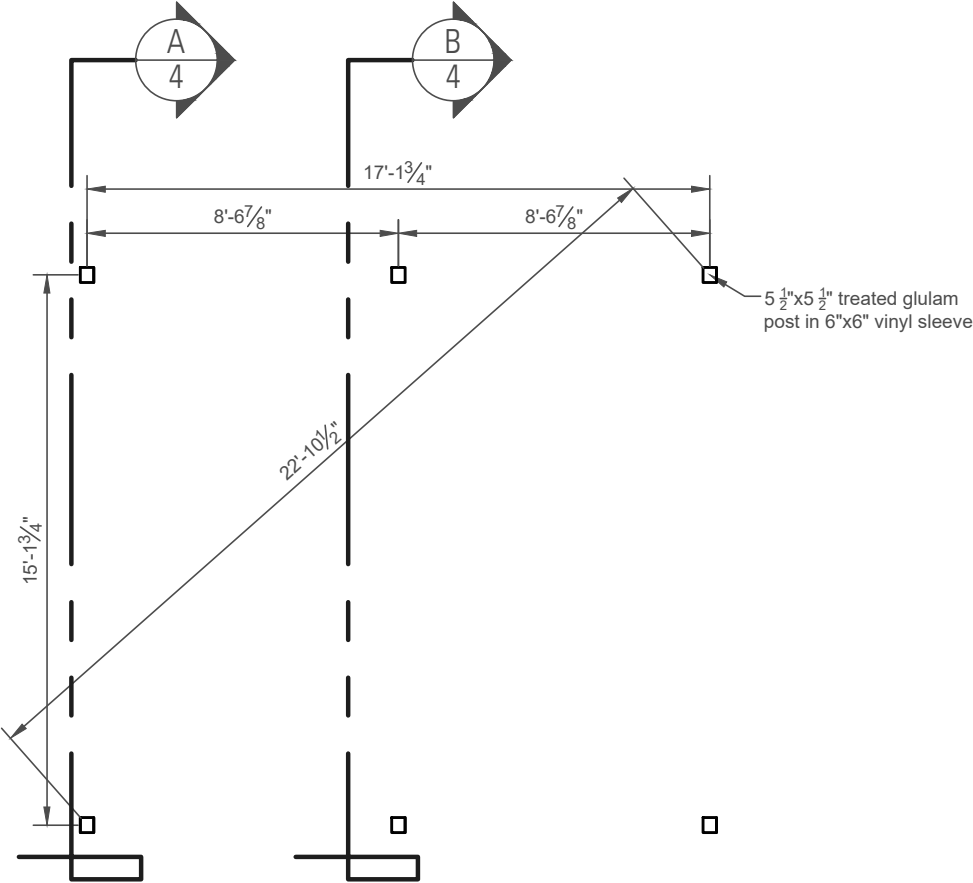
Post Layout Plan
