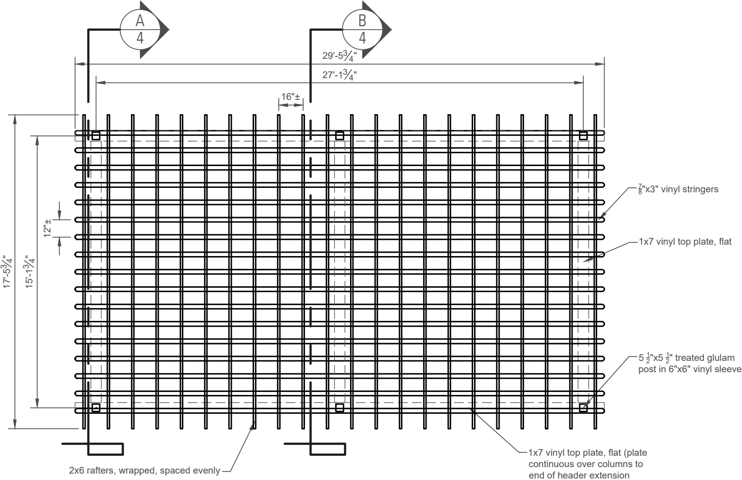
Roof Framing Plan NTS
