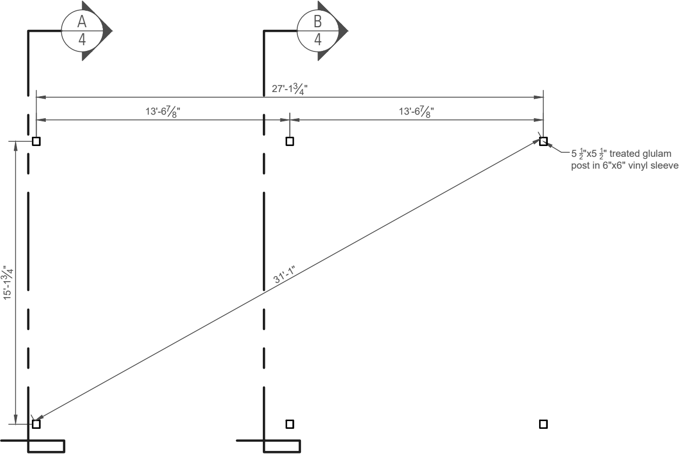
Post Layout Plan
