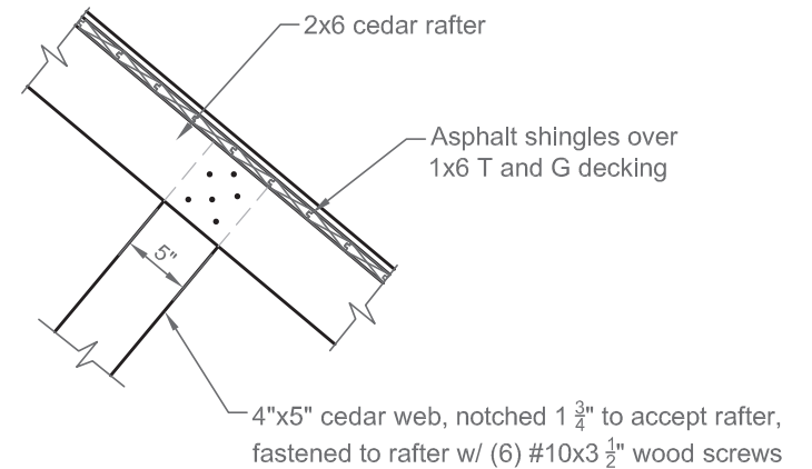
Detail B-B/4
