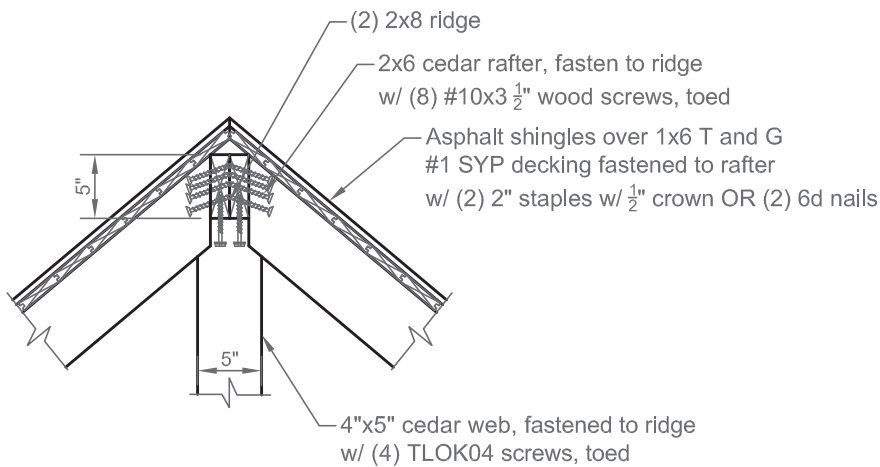
Detail A-A/4
