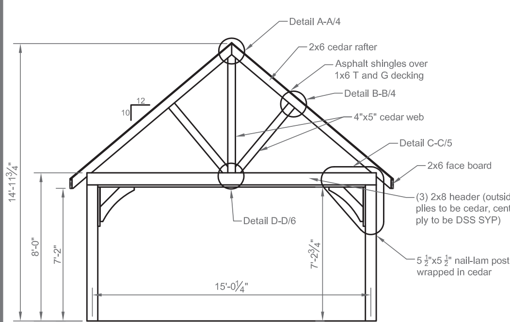
Cross Section A/4
