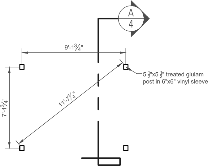
Post Layout Plan NTS
