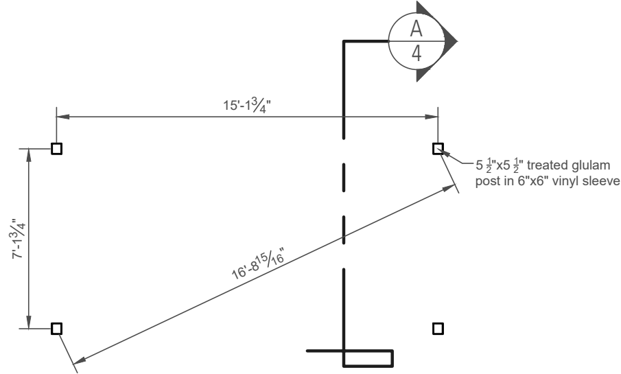
Post Layout Plan NTS
