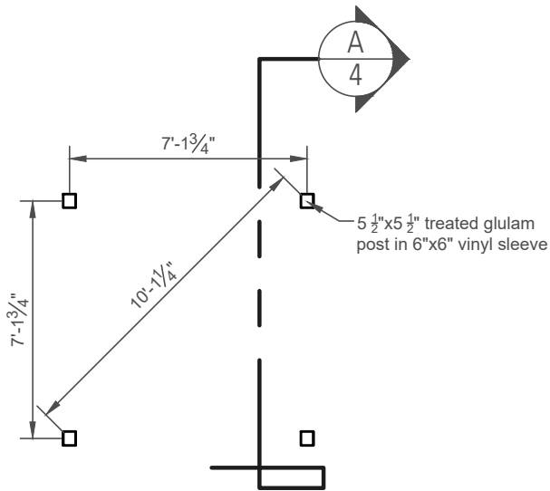
Post Layout Plan
