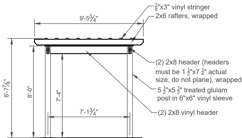
Cross Section A/4 NTS
