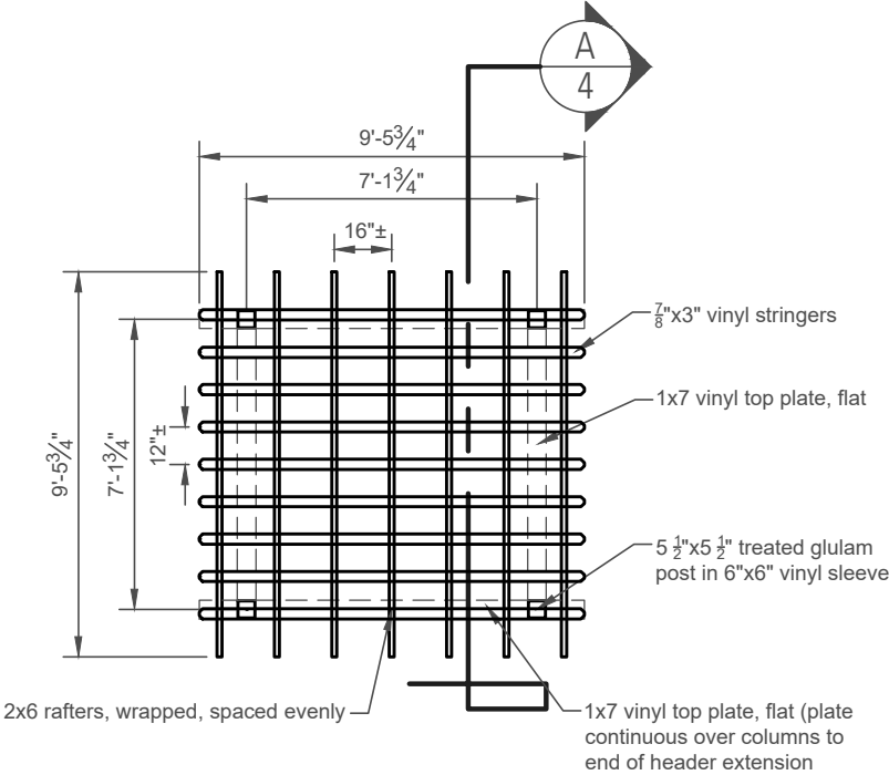
Roof Framing Plan NTS
