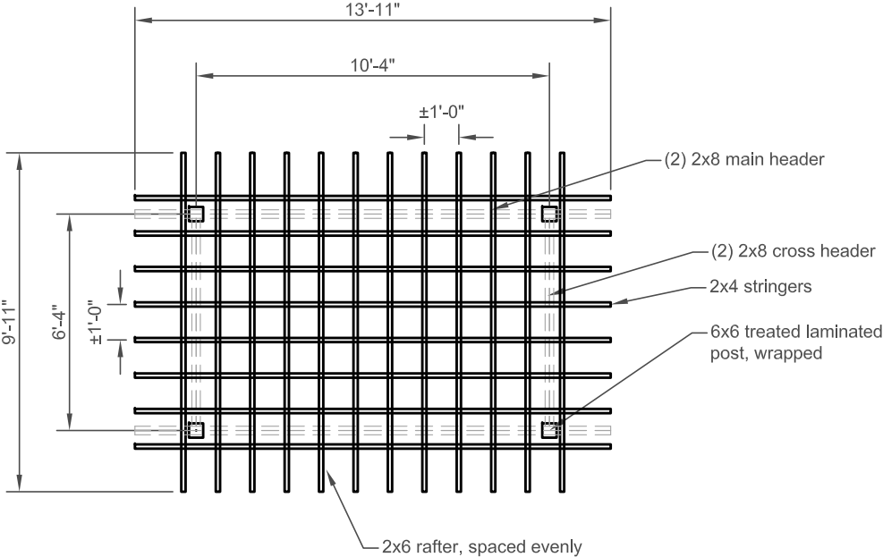
Roof Framing Plan NTS
