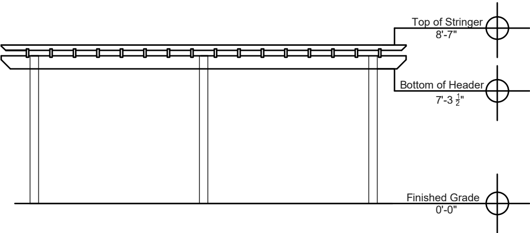
Side Elevation
