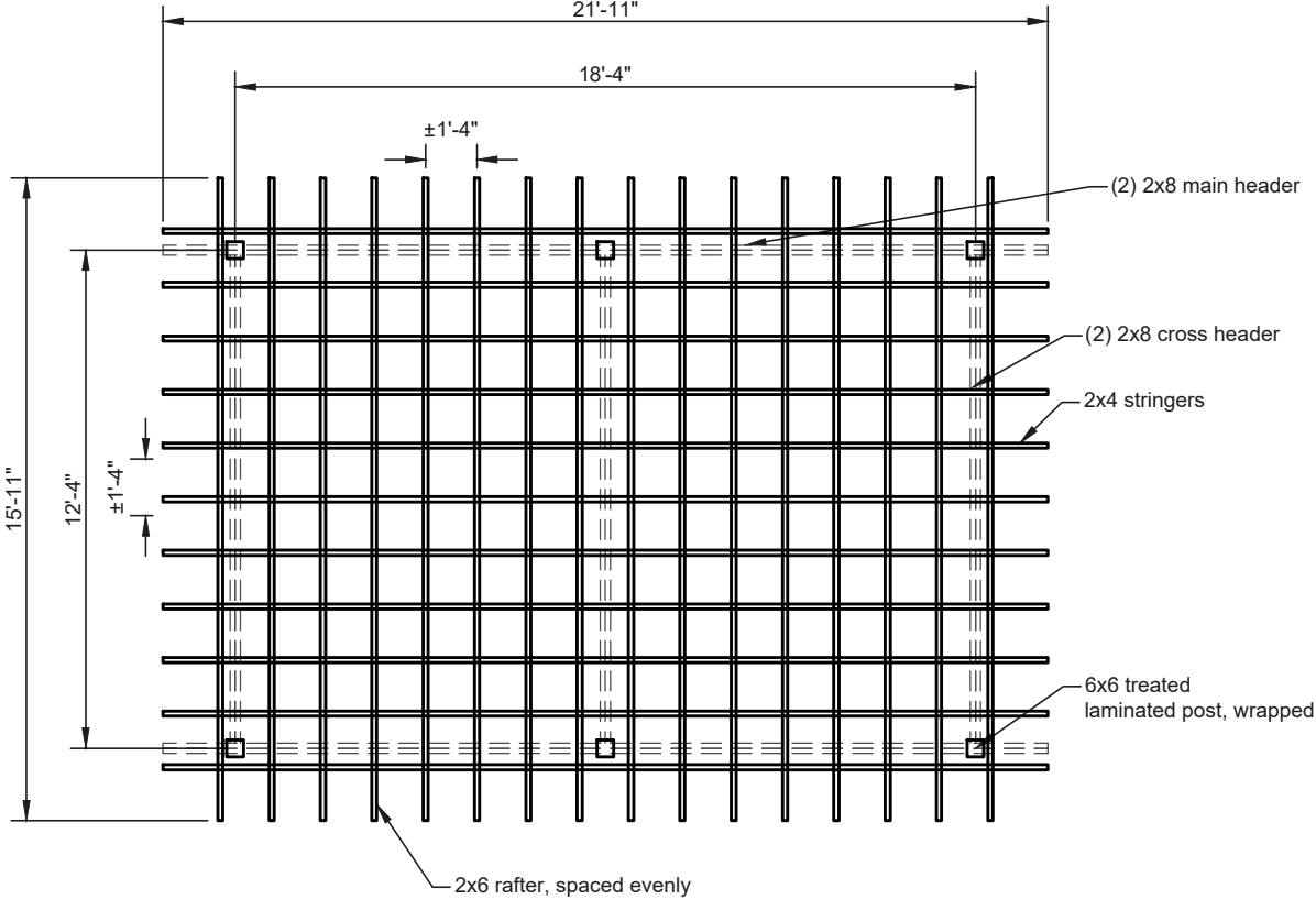
Roof Framing Plan NTS
