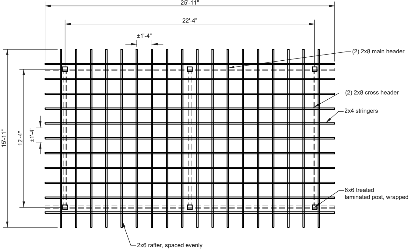
Roof Framing Plan NTS
