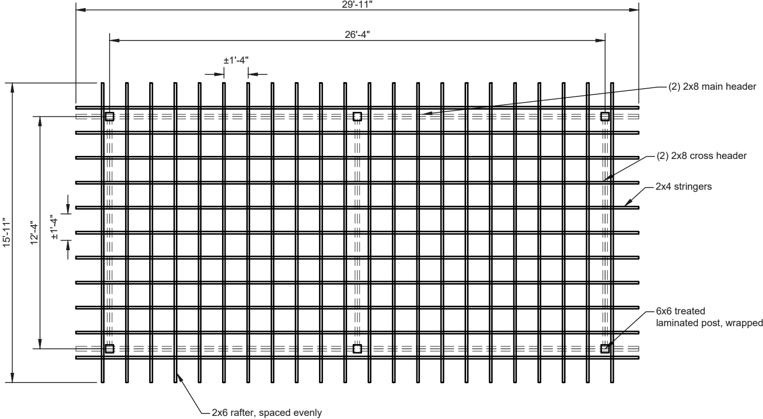
Roof Framing Plan NTS
