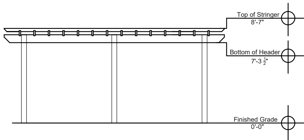
Side Elevation
