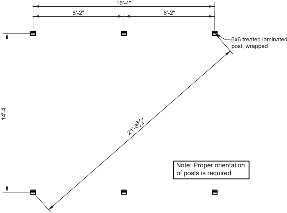
Post Layout Plan NTS
