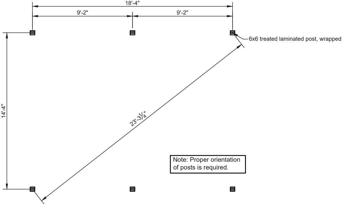
Post Layout Plan NTS
