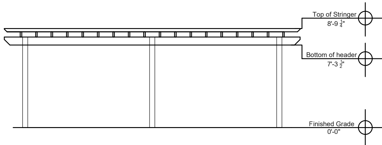
Side Elevation
