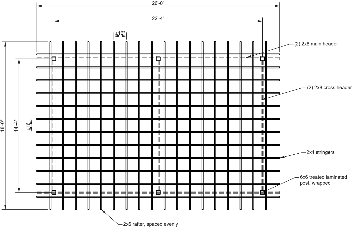
Roof Framing Plan NTS
