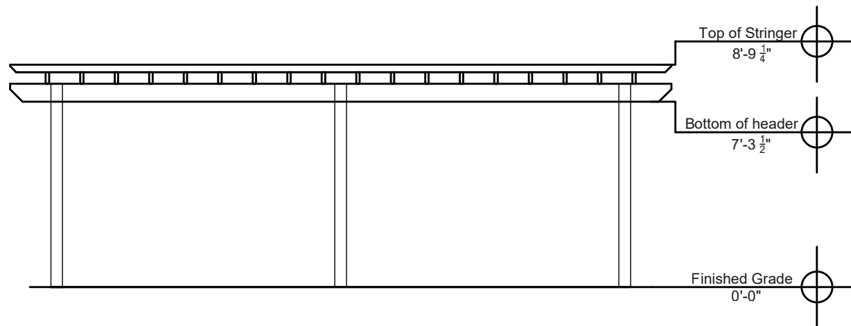
Side Elevation
