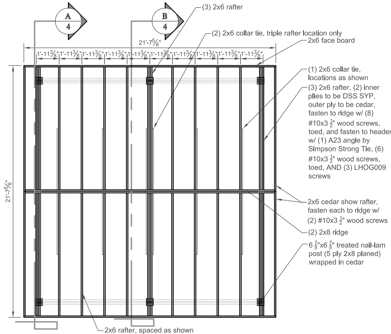
Roof Framing Plan NTS
