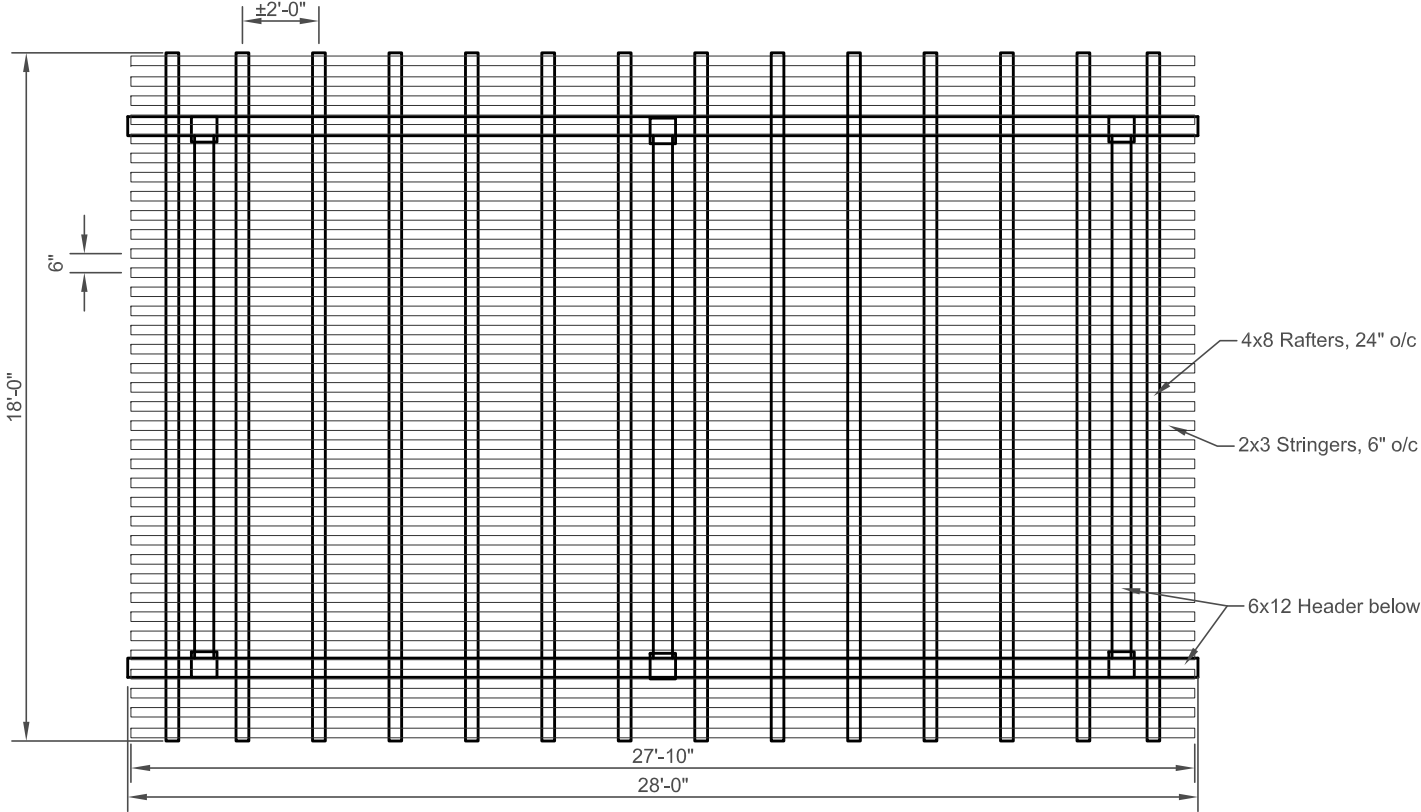
Roof Framing Plan NTS
