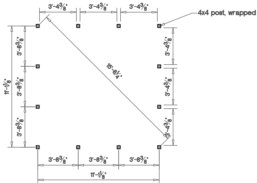
Post Layout Plan
