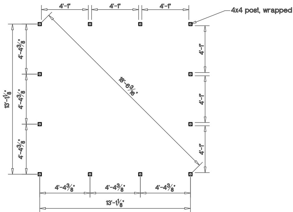
Post Layout Plan
