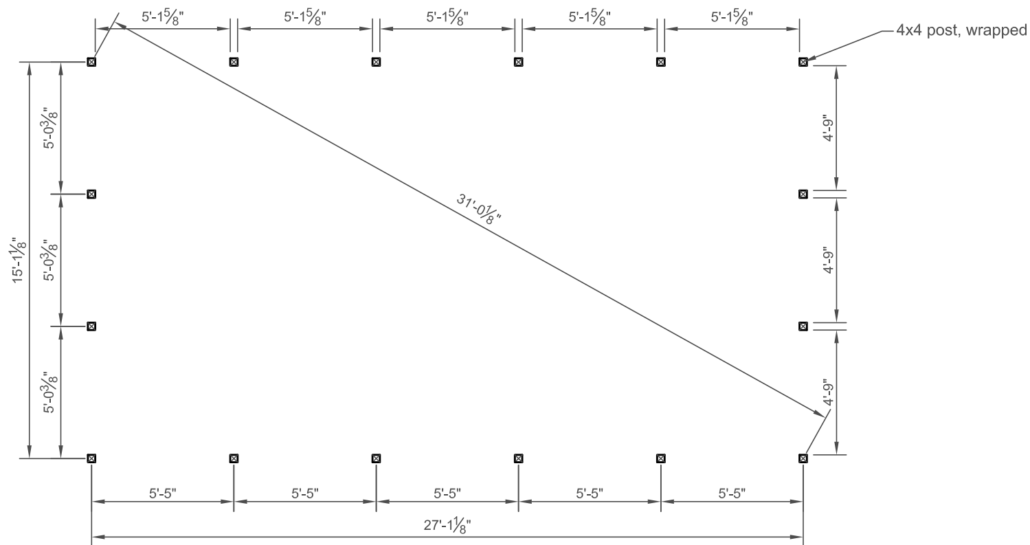
Post Layout Plan
