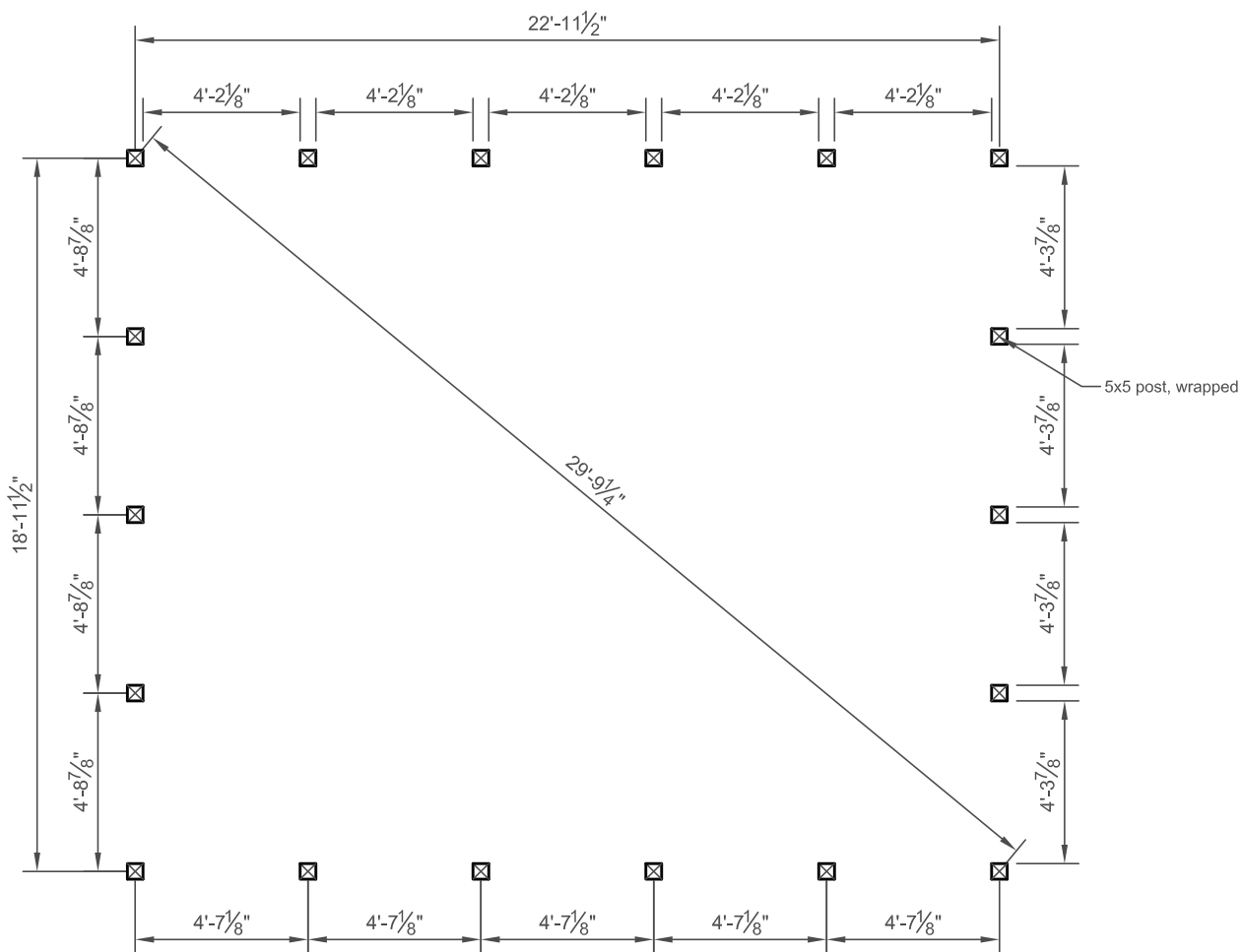
Post Layout Plan
