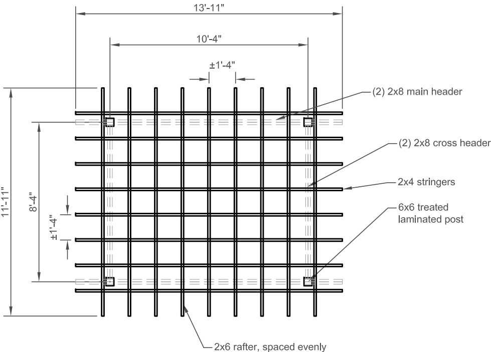
Roof Framing Plan NTS
