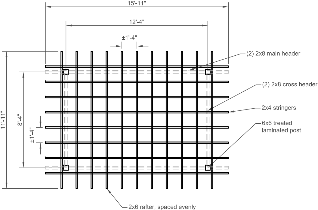
Roof Framing Plan NTS
