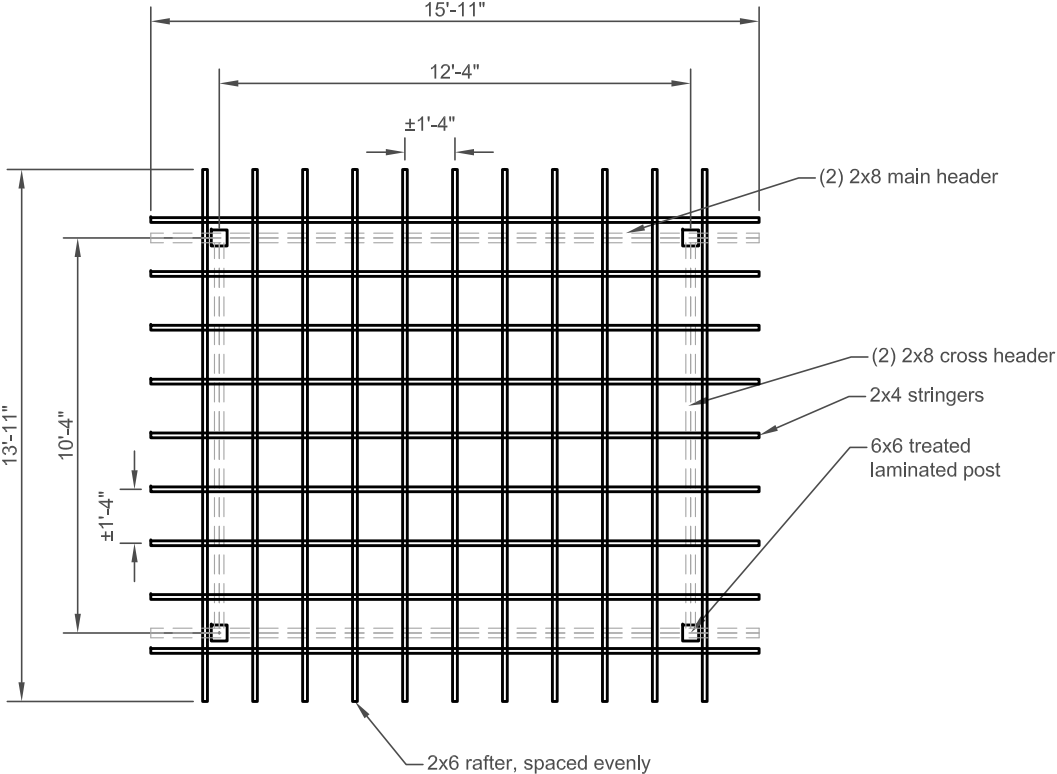
Roof Framing Plan NTS
