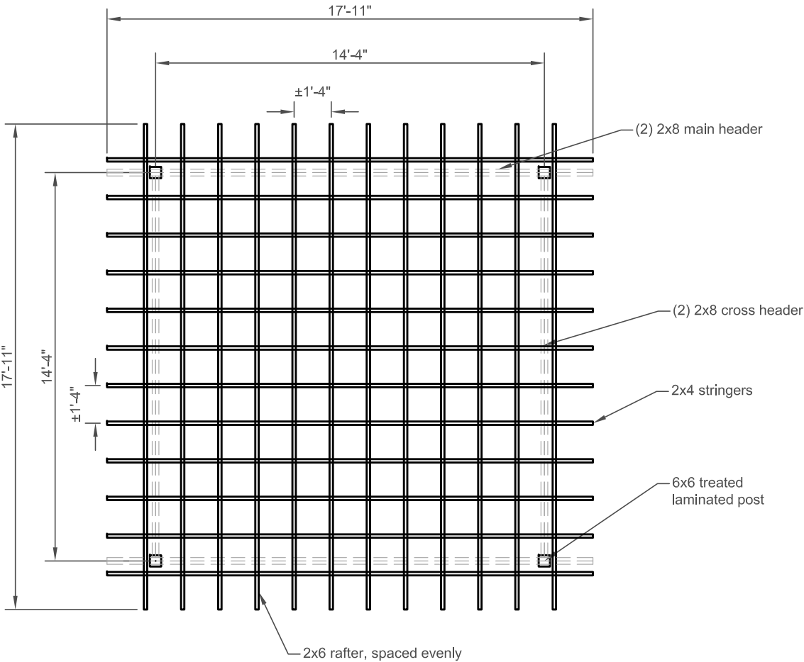
Roof Framing Plan NTS
