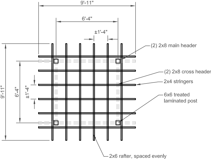
Roof Framing Plan NTS
