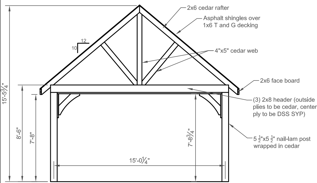
Cross Section A/4
