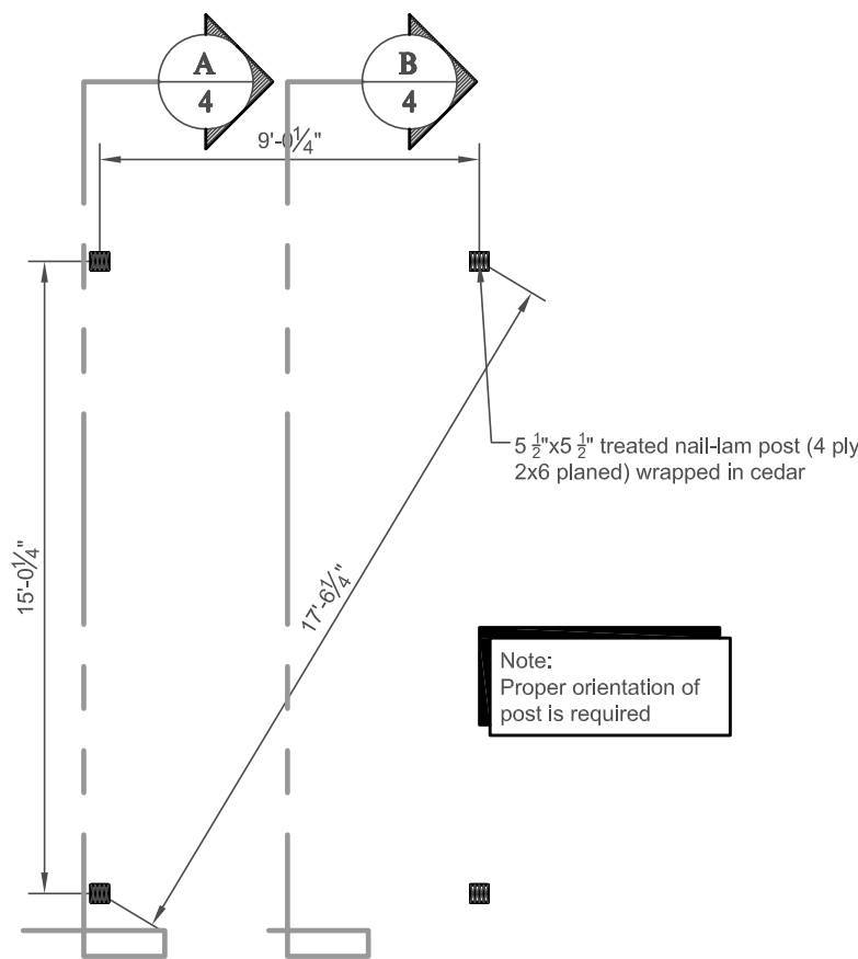
Post Layout Plan NTS
