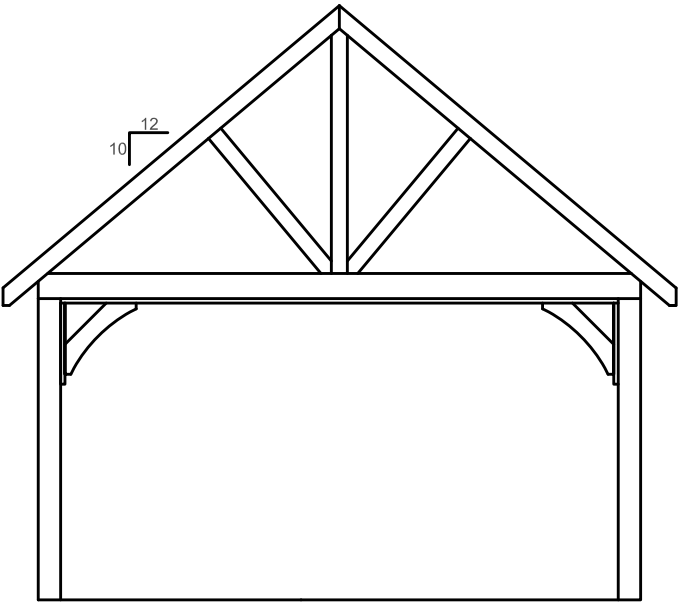
End Elevation NTS
