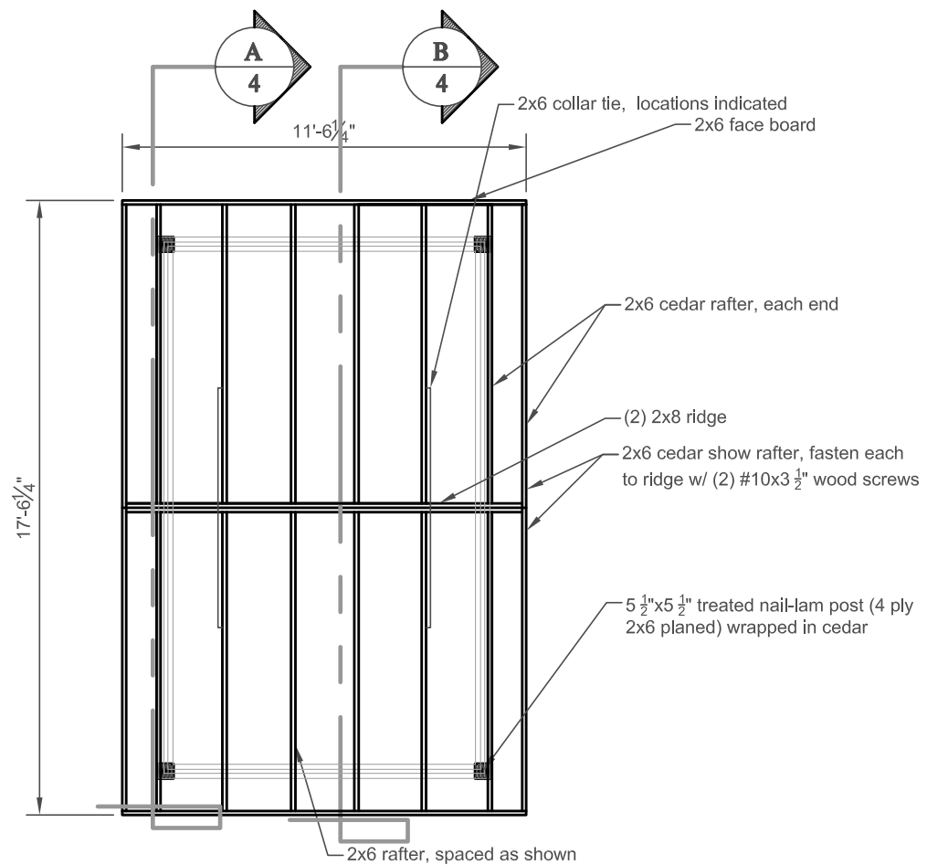
Roof Framing Plan NTS
