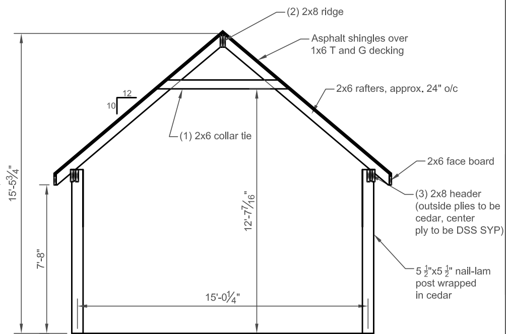
Cross Section B/4 NTS
