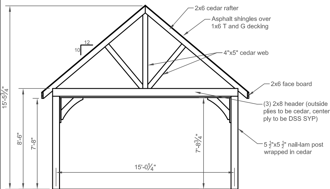
Cross Section A/4 NTS
