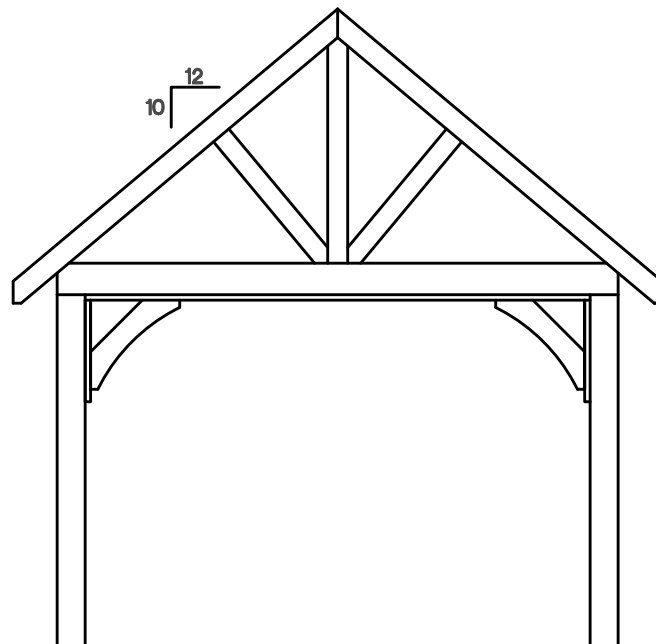
Side Elevation
