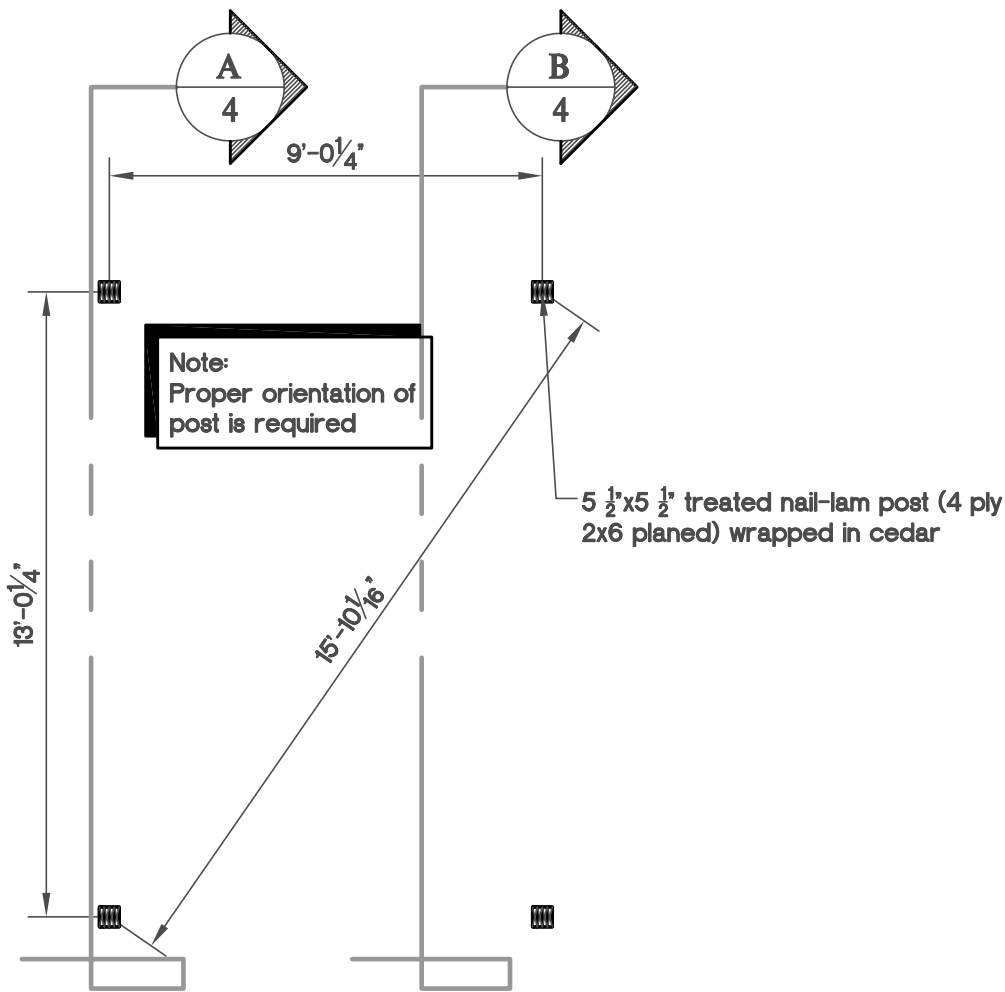
Post Layout Plan Scale 1/4" = 1'-0"
