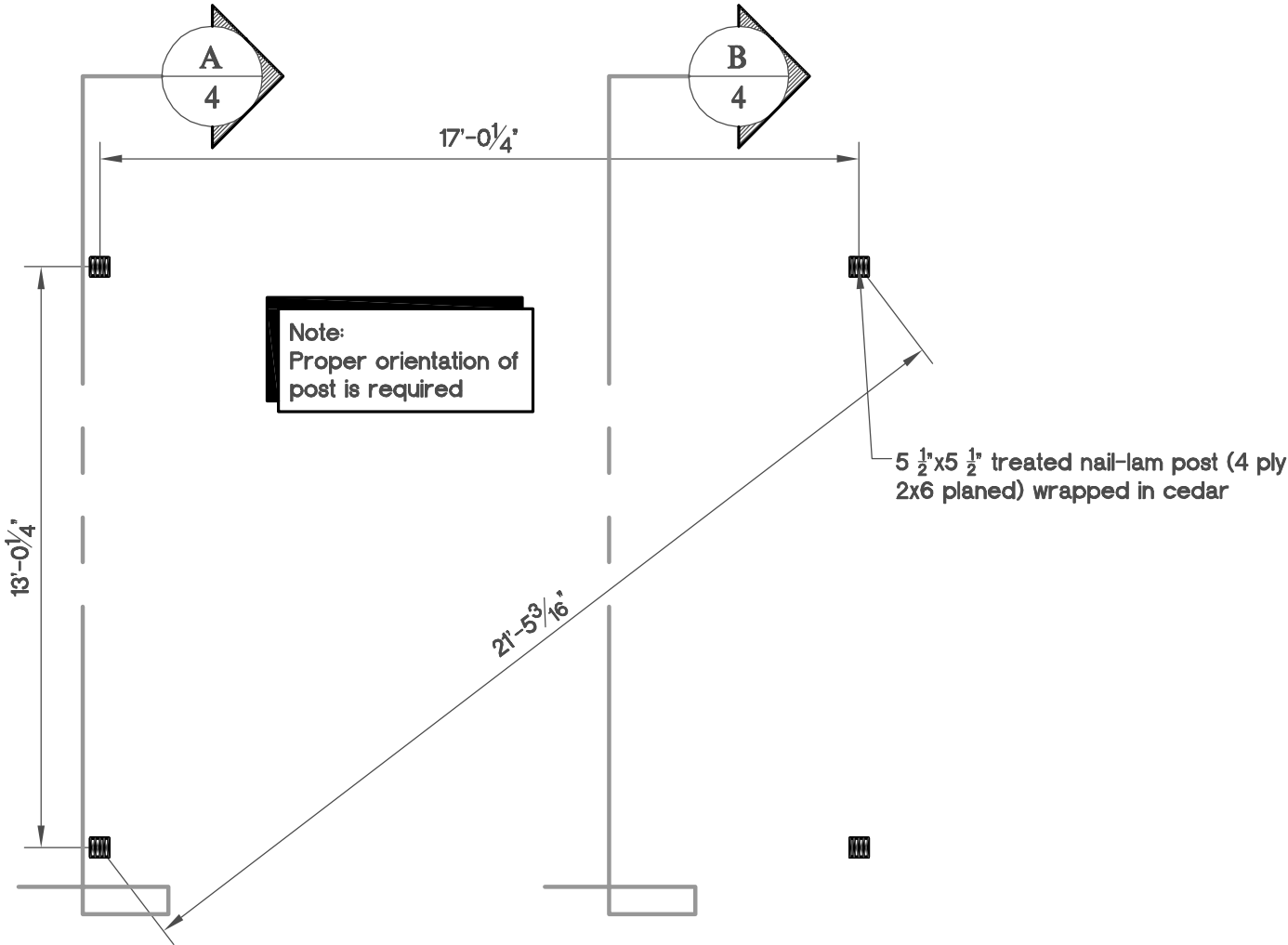
Post Layout Plan Scale 1/4" = 1'-0"
