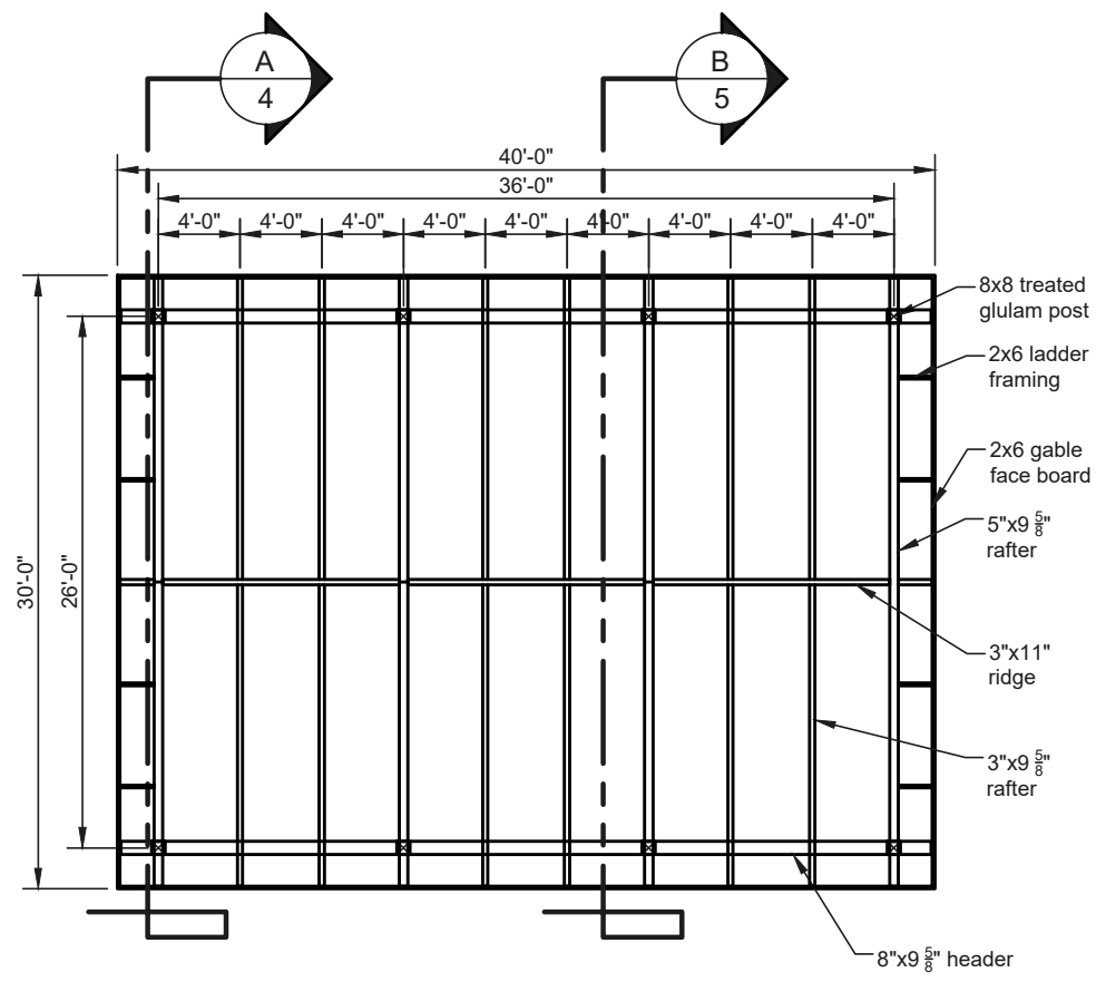
Roof Framing Plan NTS
