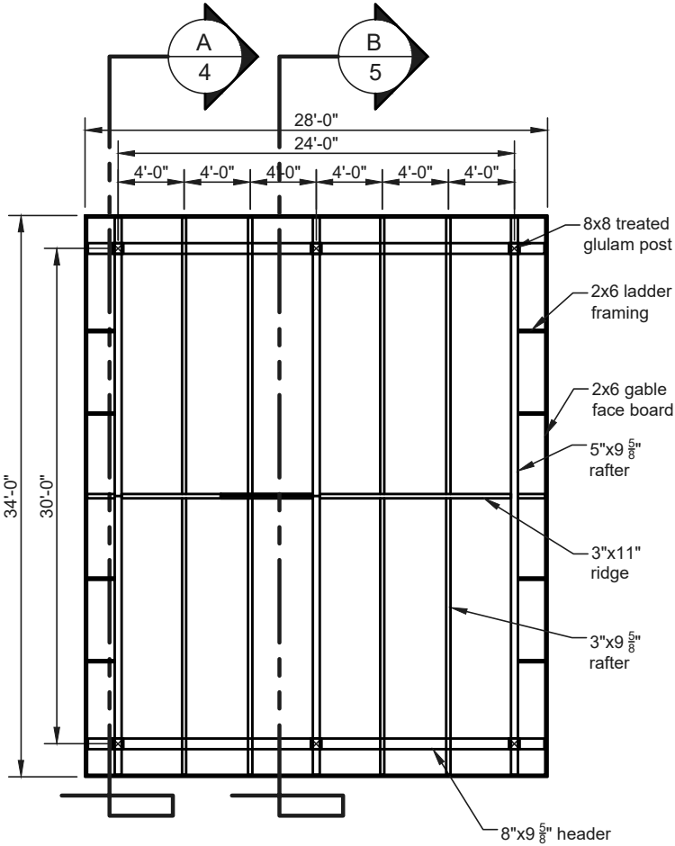
Roof Framing Plan NTS
