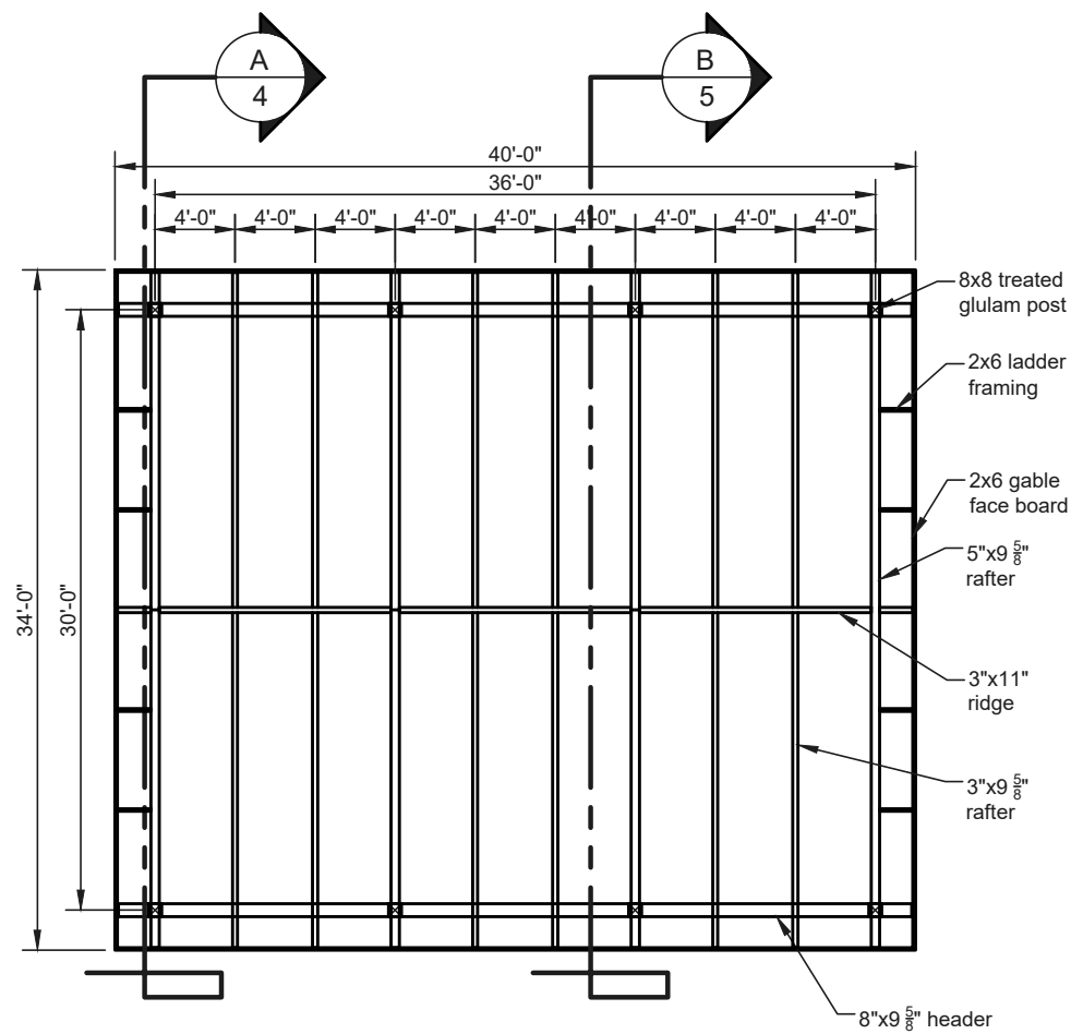
Roof Framing Plan NTS
