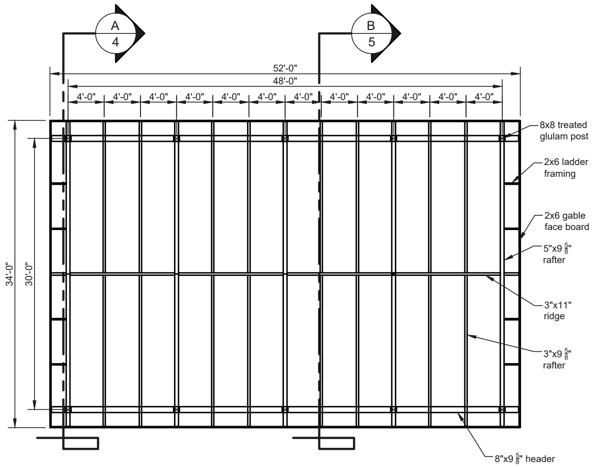
Roof Framing Plan NTS
