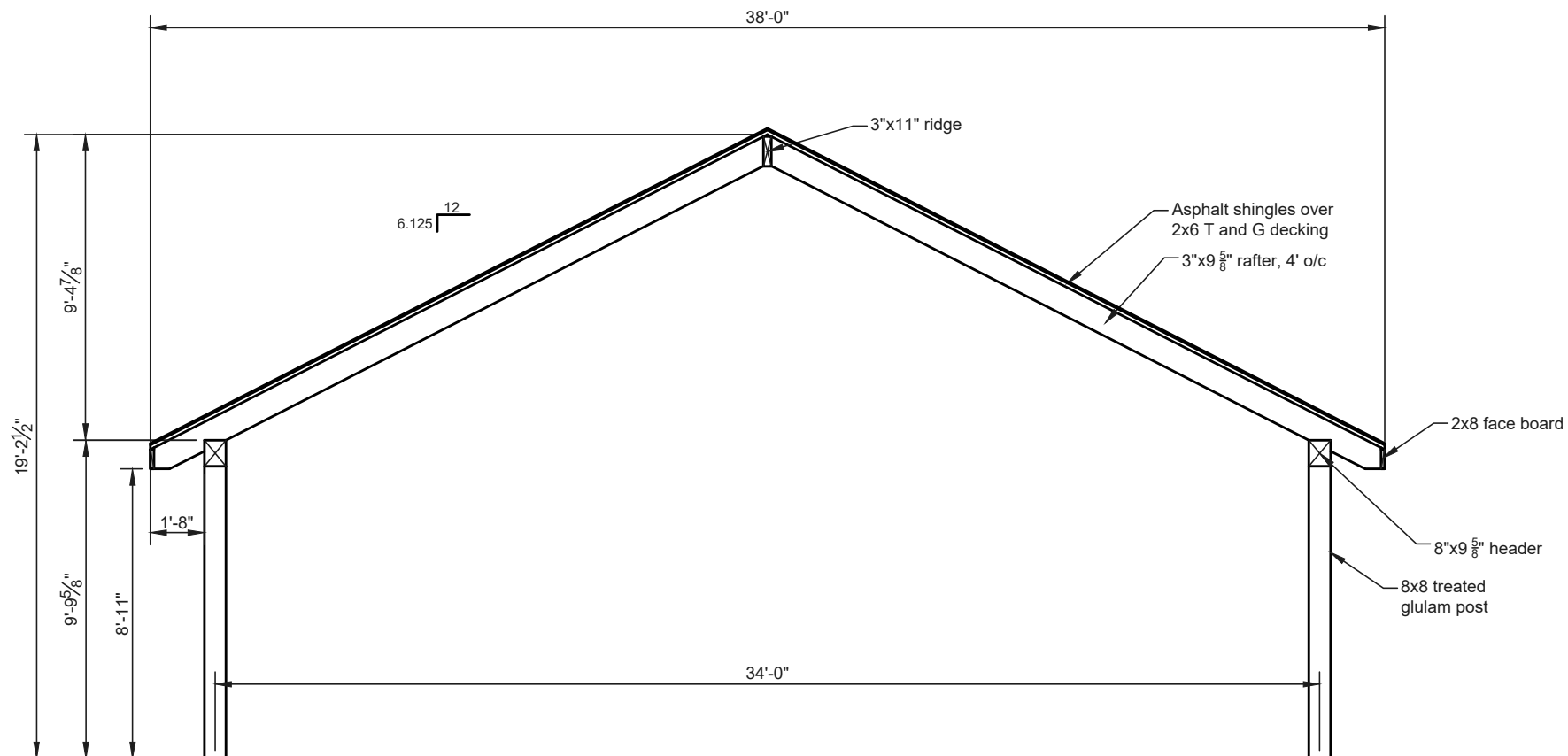
Cross Section B/5
