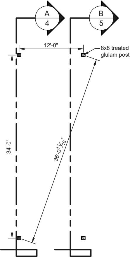
Post Layout Plan NTS
