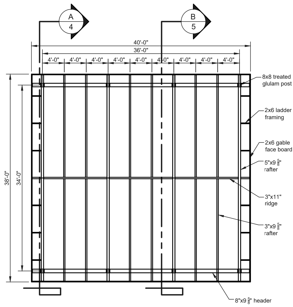
Roof Framing Plan NTS
