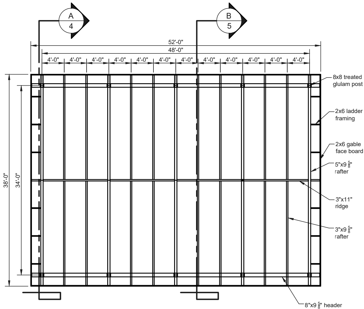
Roof Framing Plan NTS
