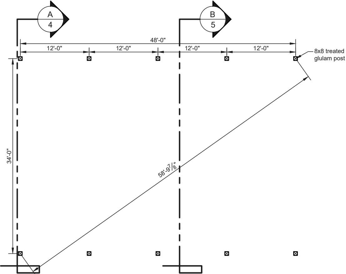
Post Layout Plan NTS
