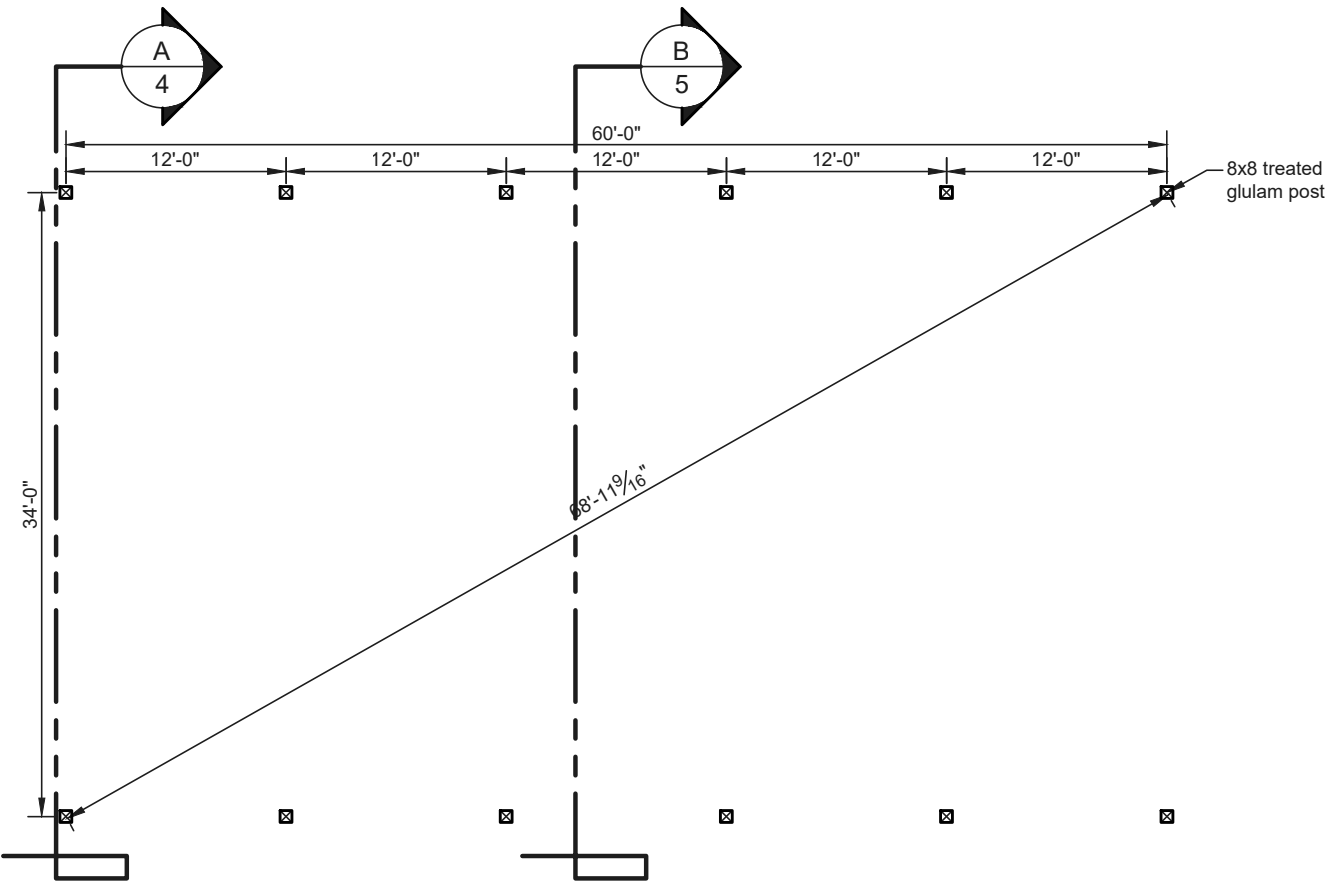
Post Layout Plan NTS
