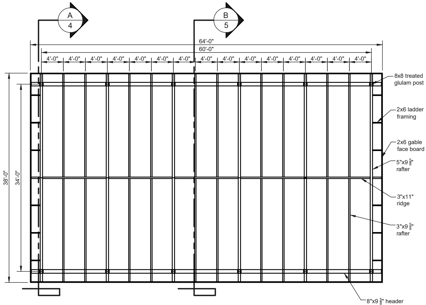
Roof Framing Plan NTS
