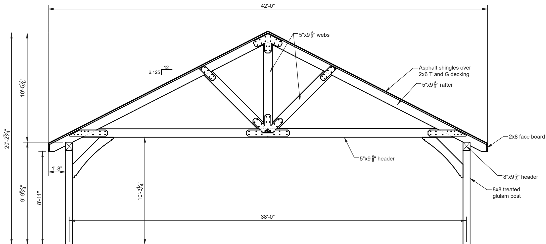
Cross Section A/4
