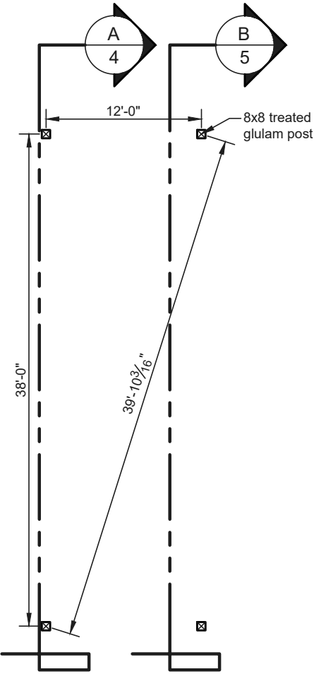
Post Layout Plan NTS
