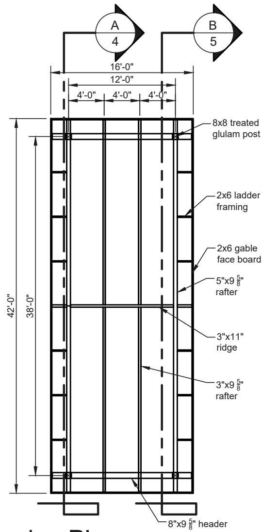
Roof Framing Plan NTS
