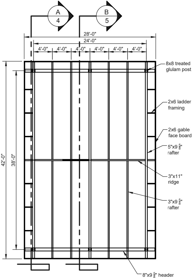
Roof Framing Plan NTS
