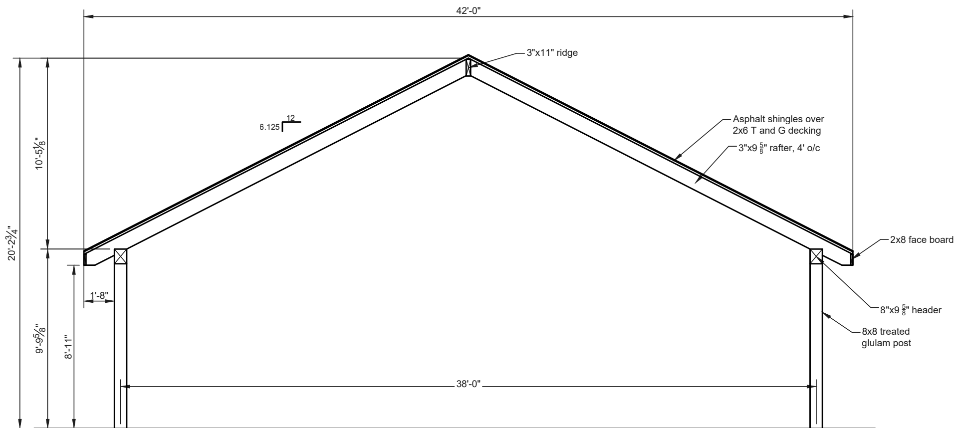
Cross Section B/5
