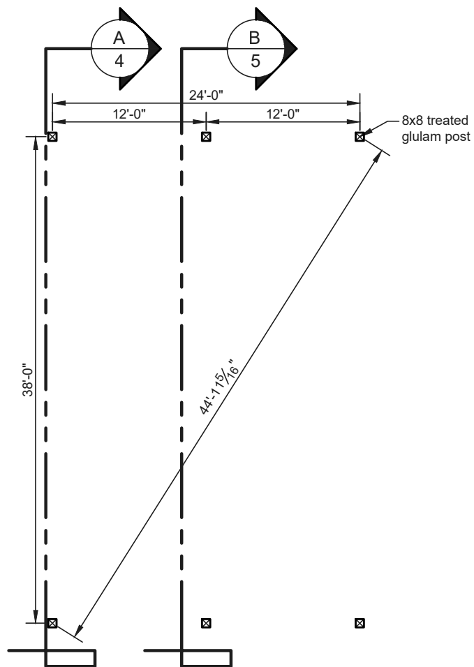
Post Layout Plan
